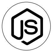
Node
