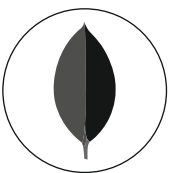
Mongo
