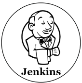
Jenkins
