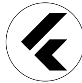
Google Flutter
